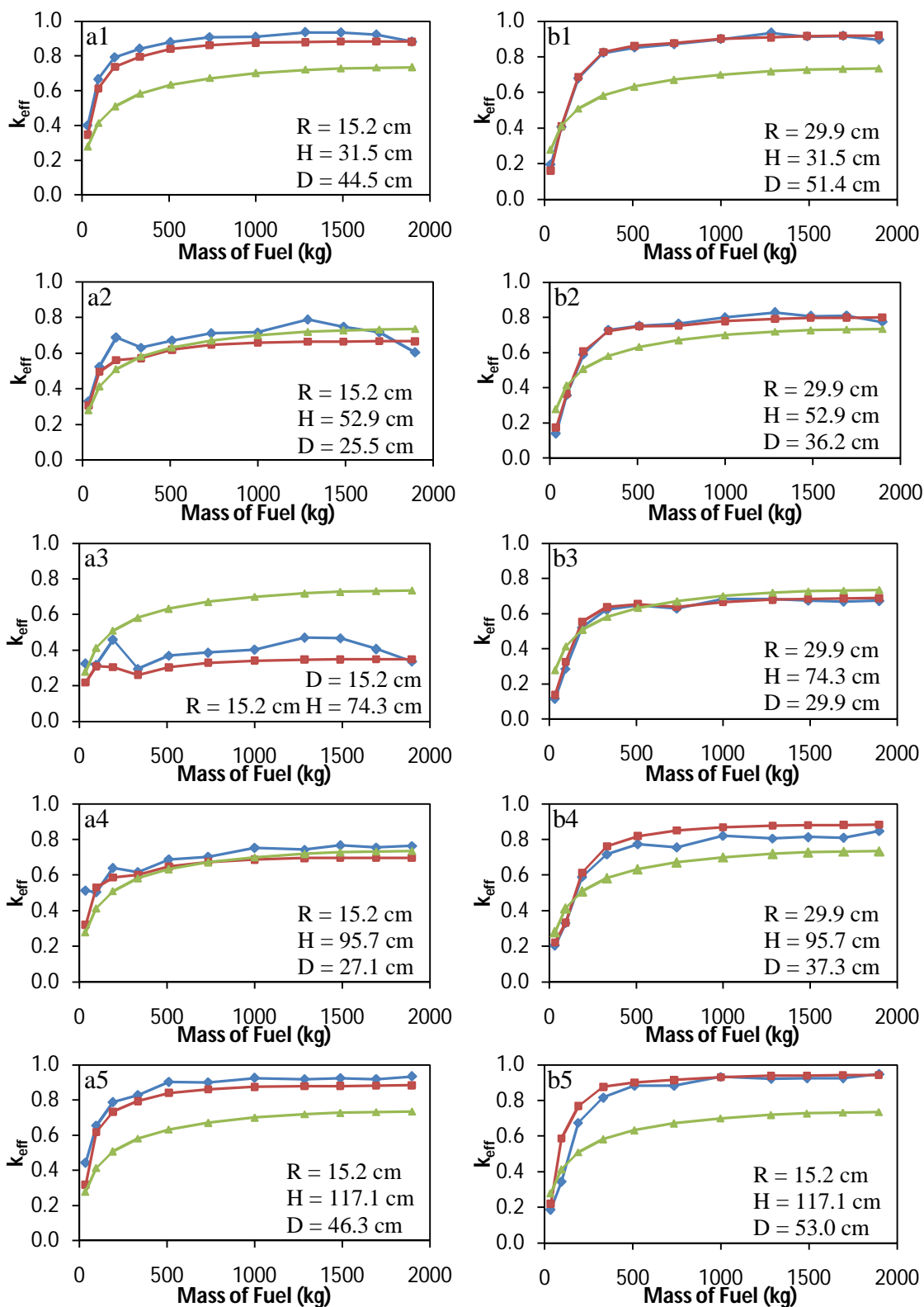
Fig. 9. Comparison of results for k_{eff} . —◆— 1/M approximation from measured values, —■— 1/M approximation from MCNP tallies, —▲— MCNP KCODE results. Radial (R) and axial (H) location is included with the distance from the detector to the neutron source (D).
