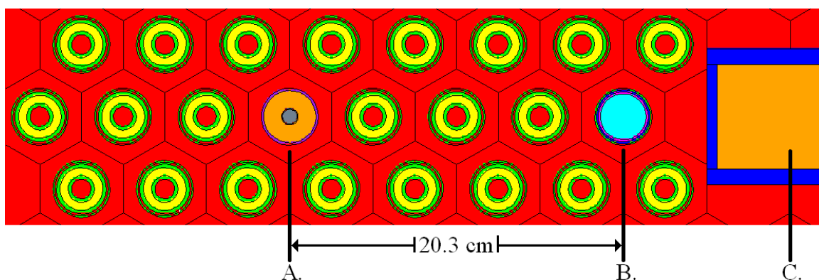
Fig. 11. Relevant geometry for the axial flux profile experiment. A. Movable detector tube. B. Pu-Be neutron source. C. Fixed detector tube
