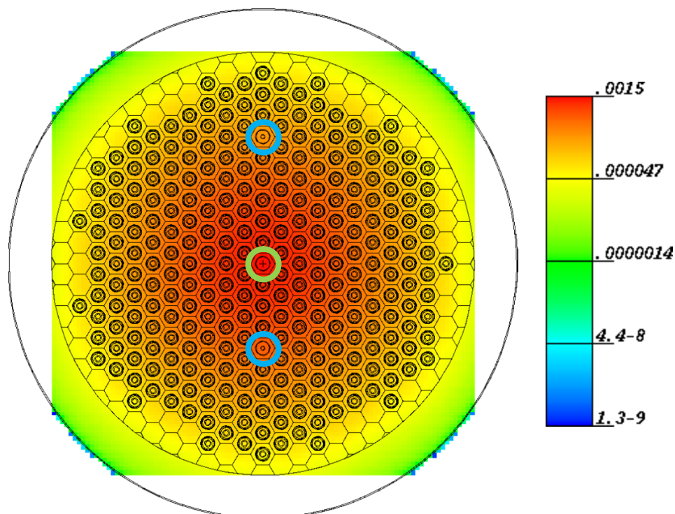
Fig. 18. Neutron flux distribution ( \text{n cm}^{-2} \text{sp}^{-1} ) 51.64 cm from the tank bottom for recommended configuration 1. Detectors are circled in blue. Source is circled in green.
